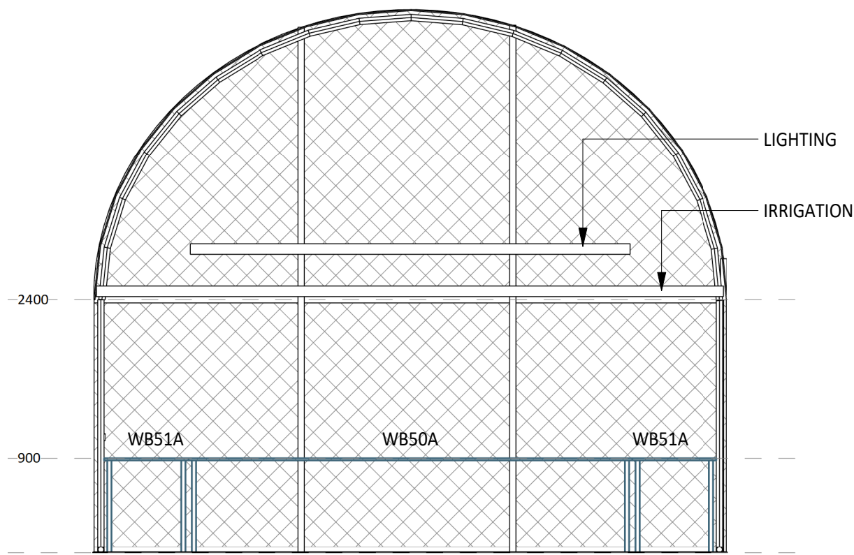
4 ELEVATION DETAIL 60-007 1 : 50
