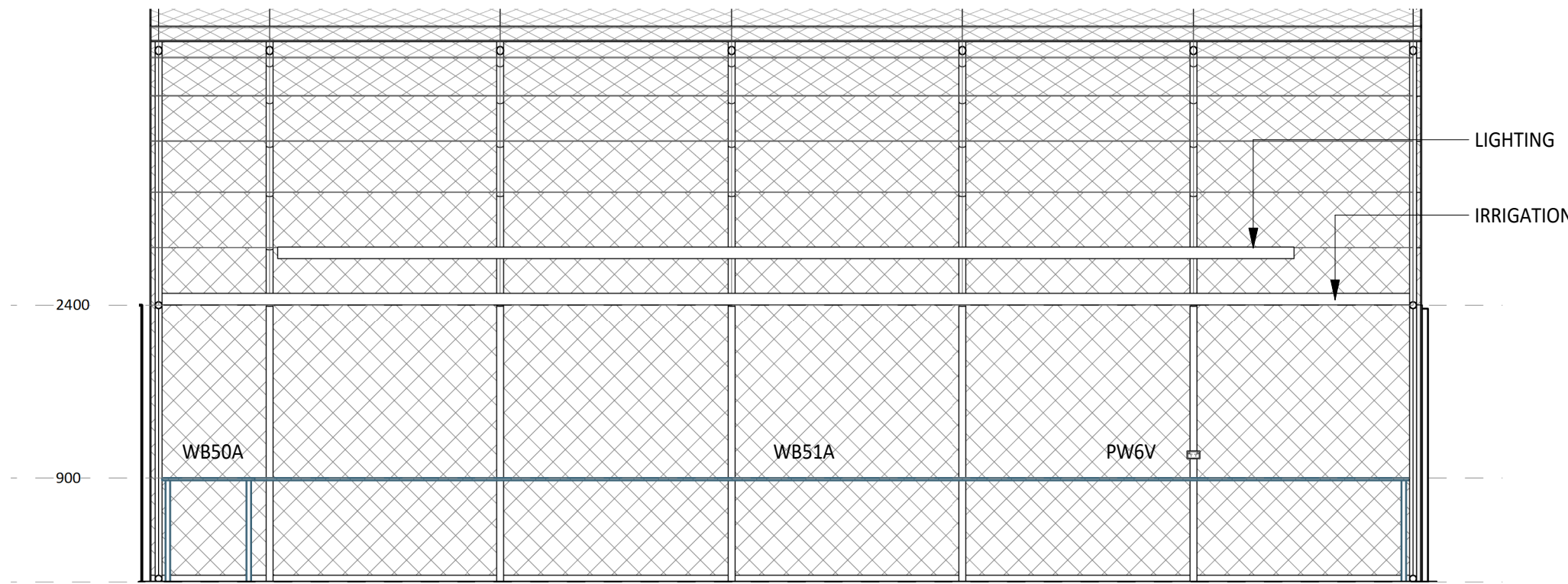
3 ELEVATION DETAIL 60-007 1 : 50
